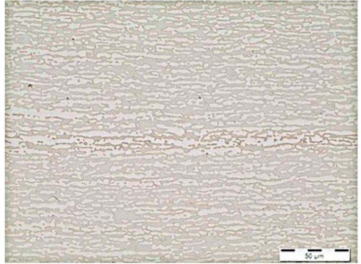
Example of the microstructure observed at mid thickness of the DX2507 (ferrite in grey, austenite in white) - no intermetallic phases detected.
