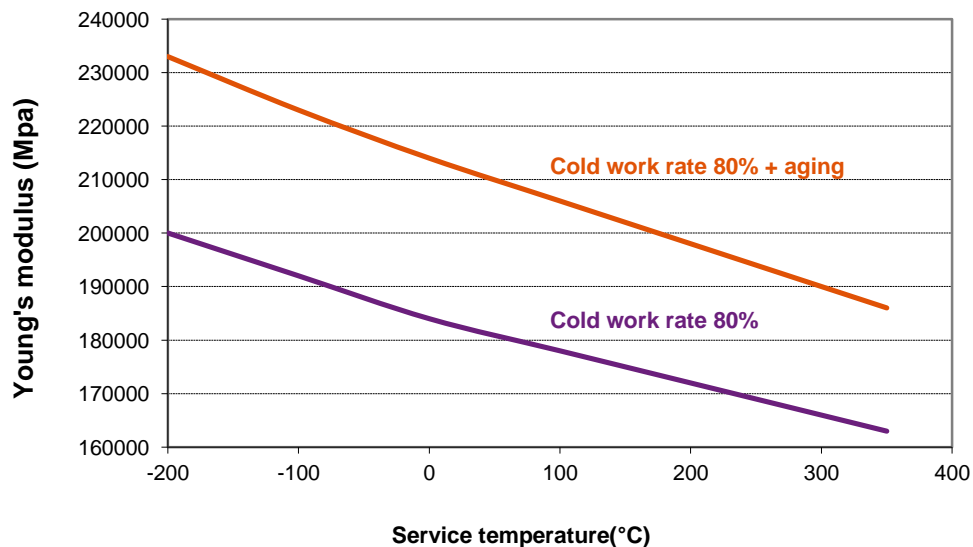
Figure 4 : Influence of service temperature on Young's modulus
