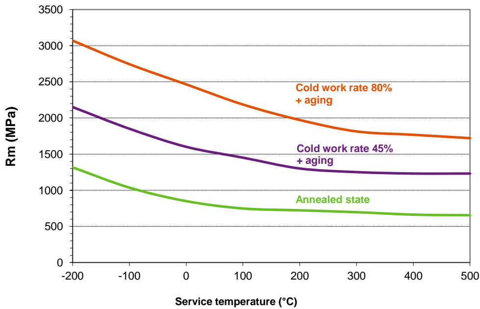
Figure 3 : Influence of service temperature on ultimate tensile strength
