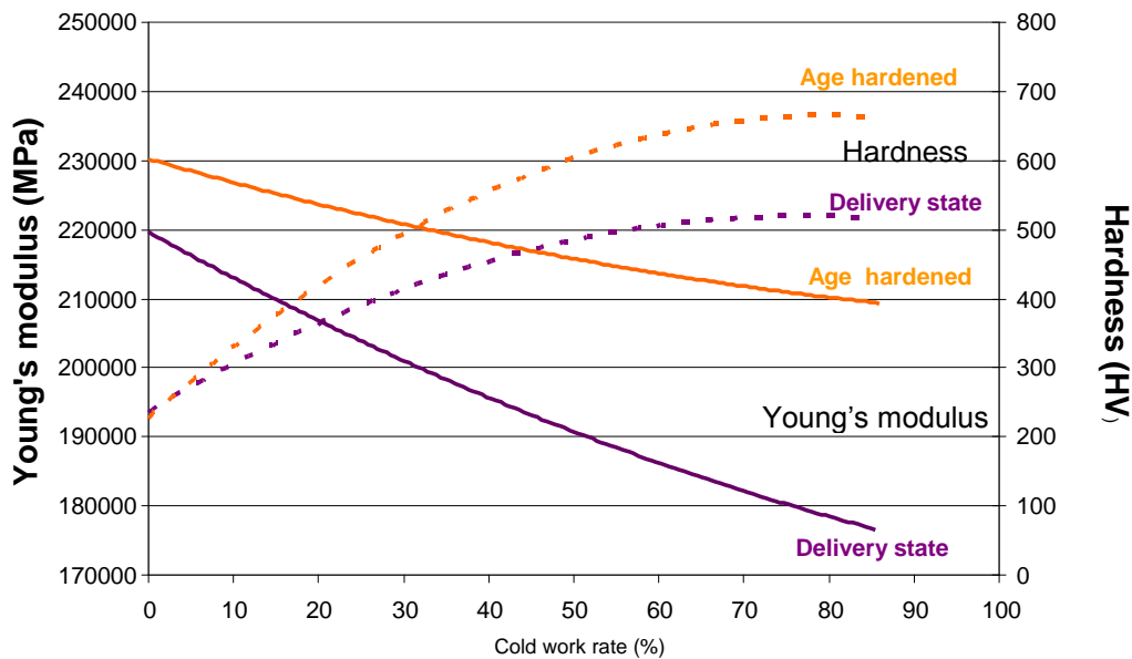
Figure 2 : Influence of the degree of cold work on the Young's modulus and hardness
